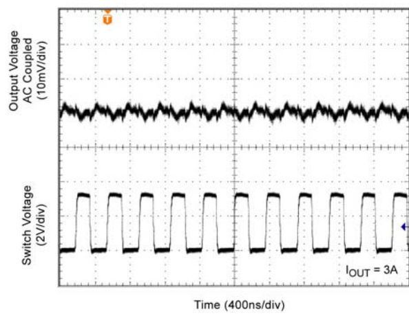
Output Ripple
